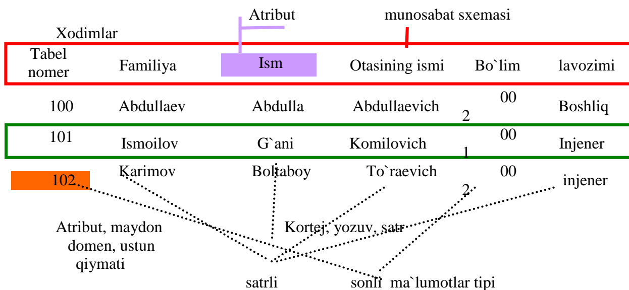
4.1.1-rasm. “Xodimlar” relyatsion modeli
