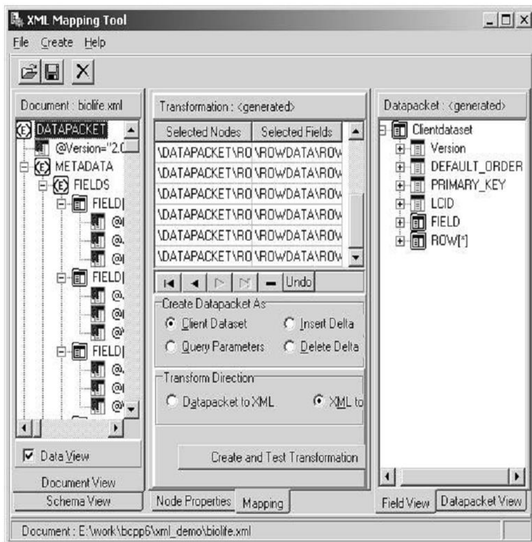
10.6.1-rasm. XML Mapping Tool oynasi
