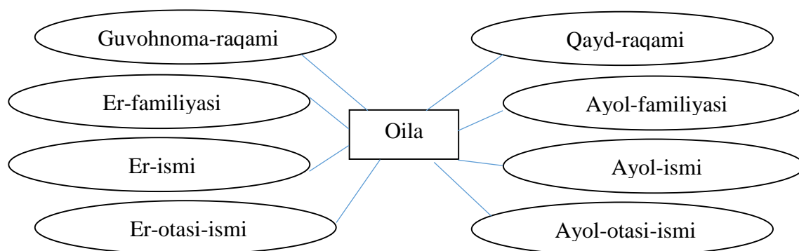
2.4.5-rasm. Oila mohiyati uchun ER diagramma
