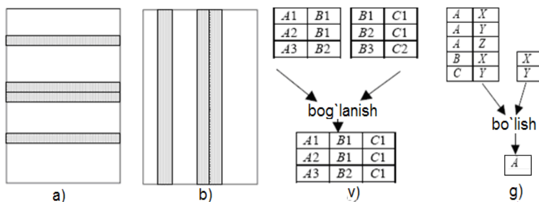
4.3.2-rasm. Maxsus relyatsion bog'lanish.
