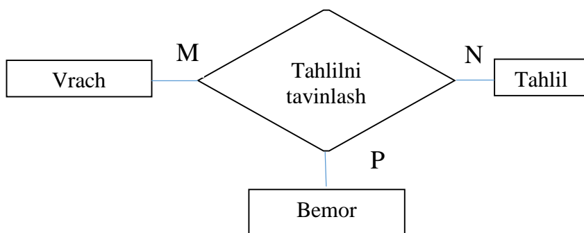
2.4.3-rasm. Trenar bog`lanish
