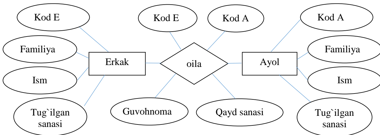
2.4.4-rasm. Oila bog`lanishining ER diagrammasi
