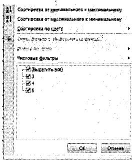
9.40-rasm. Saralash.
