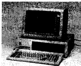
1.15-rasm. IBM-86.
