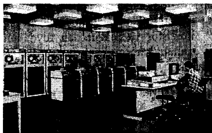
1.13 -rasm. EC- 1060.
