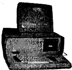
1.14-rasm. Agat.
