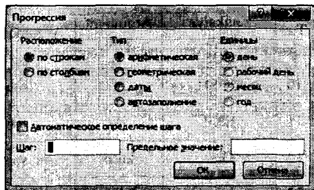
9.33-rasm. Progressiya.
