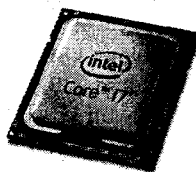
2.9-rasm. Mikroprotessor.
