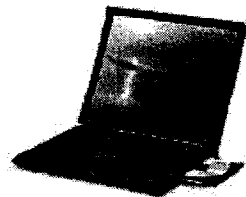
2.3-rasm. Notebook.
