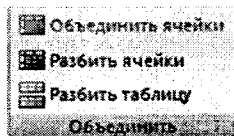
9.11-rasm. Birlashtirish.
