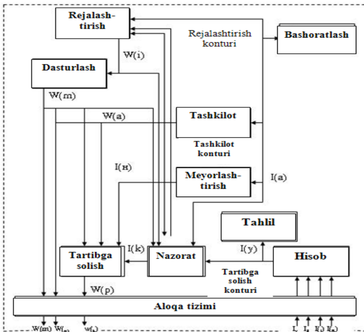
3.8 - rasm. Boshqaruv tizimining modeli 11
