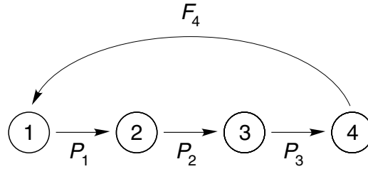
Figure 7.4. An imprimitive life cycle graph for an age-classified population with one fixed age at reproduction. The graph contains only one loop, of length 4.
