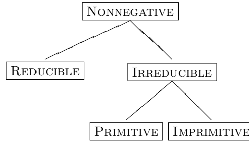
Figure 7.2. The properties of nonnegative matrices.
