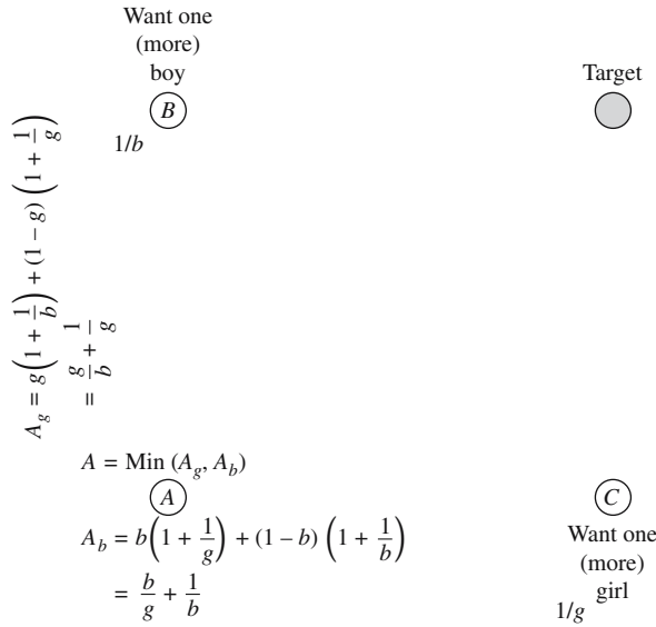
Figure 16.5. Enlargement of part of Figure 16.4, showing expected children for couple wanting one boy and one girl (position A). Trying for a boy first gives an expected A_b = b(1 + 1/g) + (1 - b)(1 + 1/b) = b/g + 1/b children. Trying for a girl first gives A_g(1 + 1/b) + (1 - g)(1 + 1/g) = g/b + 1/g children, where b is the chance of having a boy if the couple try for a boy, and g is the chance of having a girl if they try for a girl.
