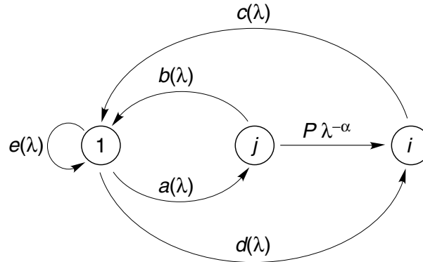
Figure 13.4. A life cycle graph for evaluating the sensitivity of \lambda to changes in \alpha , the time required for the transition from stage j to stage i .
