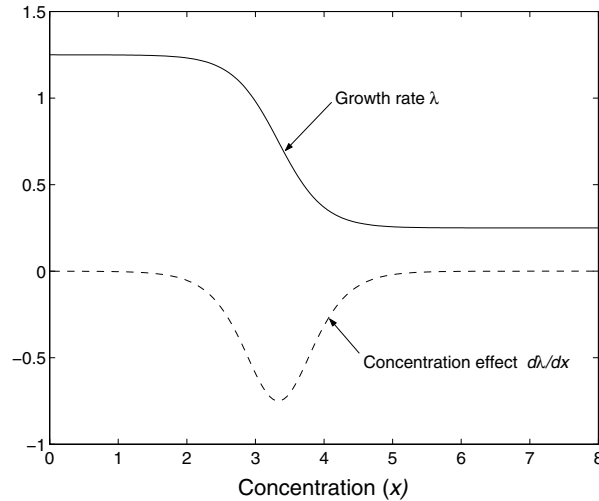
Figure 13.14. A hypothetical example showing \lambda as a function of concentration ( x ) and the effect of x , measured as the rate of change of \lambda with respect to x .
