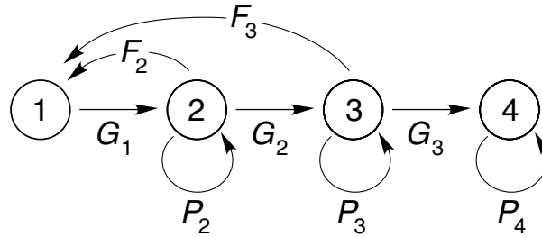
Figure 3.10. A life cycle graph for the killer whale (Brault and Caswell 1993). Nodes represent stages: \mathcal{N}_1 = yearlings, \mathcal{N}_2 = juveniles, \mathcal{N}_3 = mature females, and \mathcal{N}_4 = postreproductive females.
