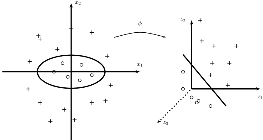
FIGURE 22.9. Kernelization. Mapping the covariates into a higher-dimensional space can make a complicated decision boundary into a simpler decision boundary.
