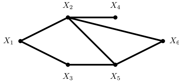
FIGURE 18.9. The maximum cliques of this graph are \{X_1, X_2\} , \{X_1, X_3\} , \{X_2, X_4\} , \{X_3, X_5\} , \{X_2, X_5, X_6\} .
