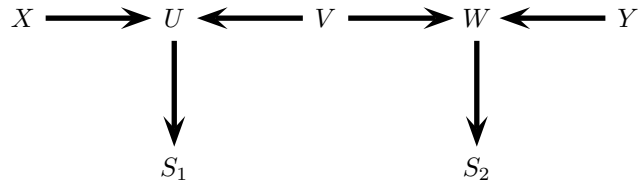
FIGURE 17.8. d-separation explained.
